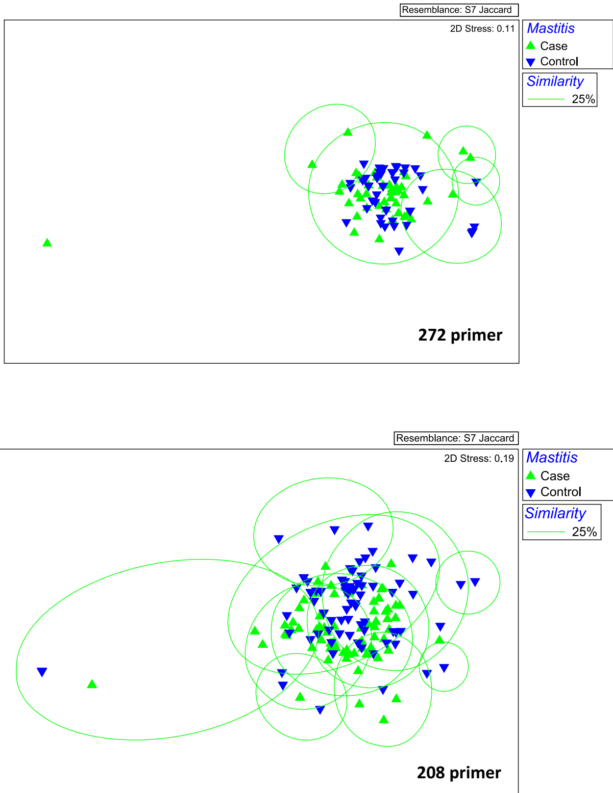
FIGURE 1 Multidimensional scaling plot of isolates based on random amplified polymorphic DNA (RAPD) profiles (272 and 208 primer) for all cases and controls.
